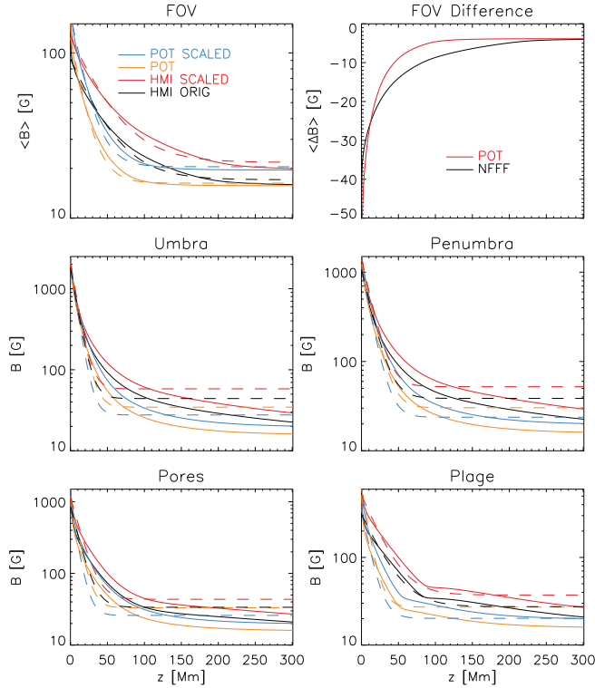
Figure 18. Average field strength with height B(z) for different structures. Left column, bottom to top: average B(z) for pores, umbra and the full FOV. Right column, bottom to top: average B(z) for plage and penumbra, and difference of average B(z) between the original and scaled HMI data across the full FOV. Black (red) lines: original (scaled) HMI data in the NFFF extrapolation. Orange (blue) lines: original (scaled) HMI data in the potential extrapolation. Dashed lines in the same colors: exponential fit.
