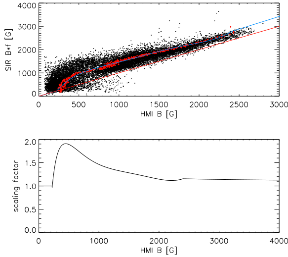
Figure 8. Scatterplot of HMI B and SP SIR Bf (top panel) and scaling curve for HMI data derived from it (bottom panel). The red pluses in the top panel are binned data points, the blue line a polynomial fit and the red solid line is at unity slope.
