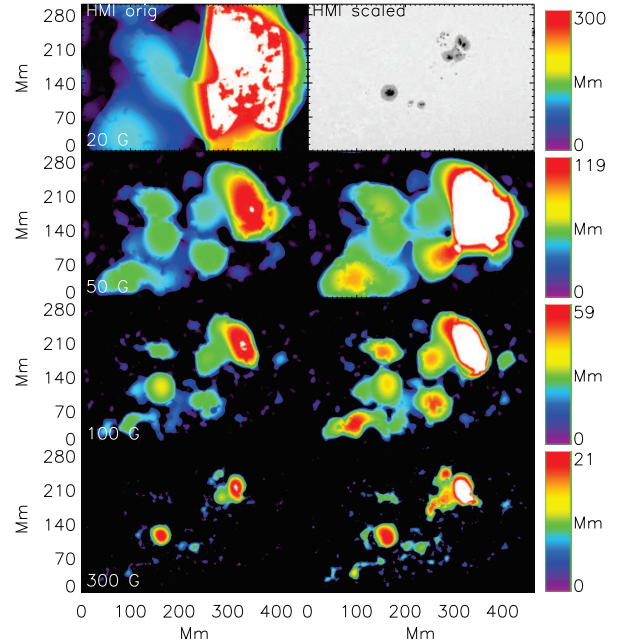
Figure 22. Height of different magnetic field strength values. Left column, bottom to top: height for B = 300, 100, 50 and 20 G in the original HMI data. Right column: the same for the scaled HMI data. The topmost panel has been replaced with the HMI continuum intensity as reference.
