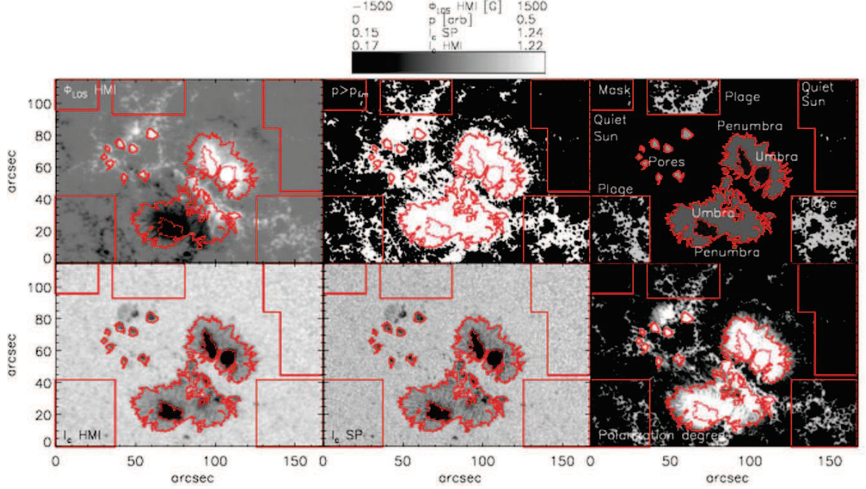
Figure 2. Overview of NOAA 12104 on 2014 Jul 03 at about UT 19:30. Bottom row, left to right: continuum intensity I_c from HMI pseudo-scan, I_c and polarization degree p from SP data. Top row, left to right: LOS magnetic flux \Phi_{LOS} from HMI, locations with p > p_{lim} in SP data, and mask of surface structures (QS to umbra from white to dark grey). Red rectangles at the corners indicate QS and plage regions, other contour lines indicate pores, penumbral and umbral regions.
