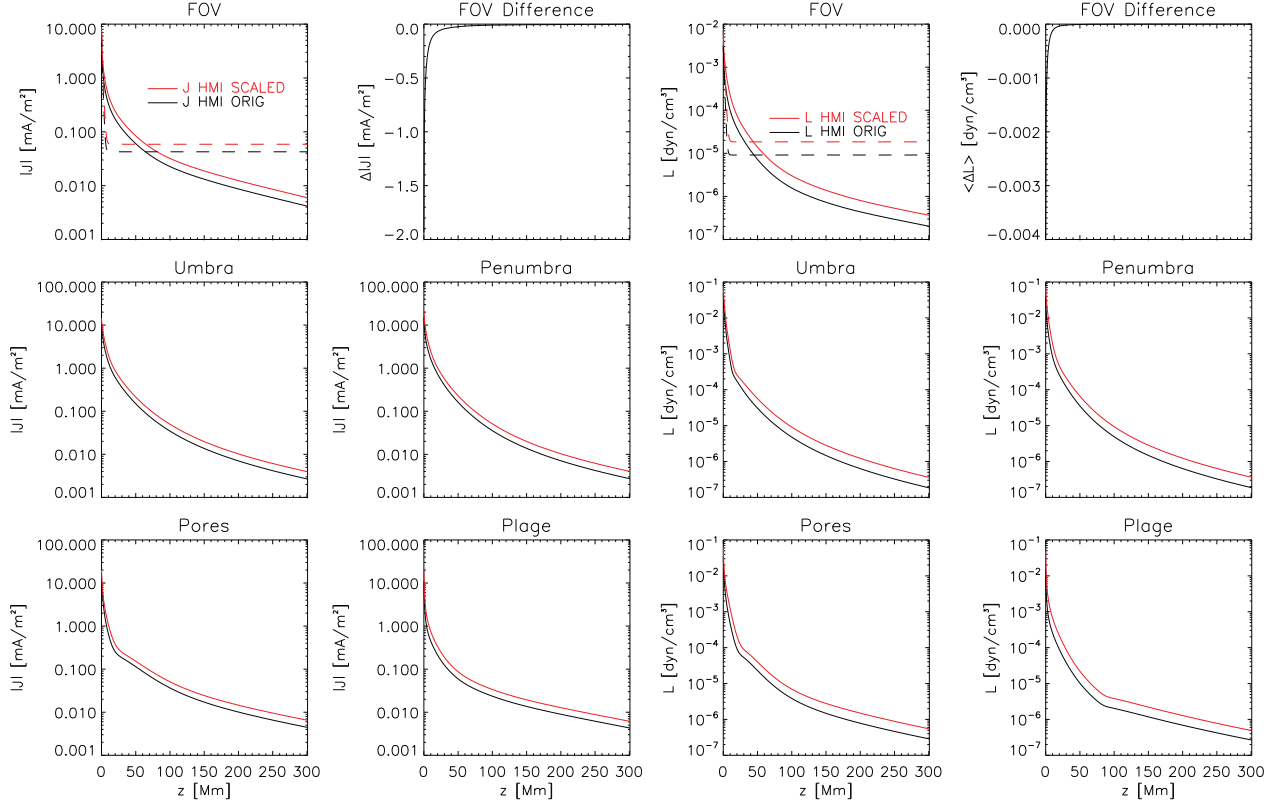
Figure 21. Average electric currents (left two columns) and Lorentz force (right two columns) in the same format as Fig. 18.
