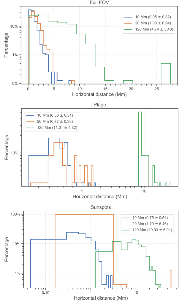
Figure 16. Horizontal distance between open field lines from the same seed point before and after the scaling at 3 heights of 10 (blue lines), 20 (orange lines), and 120 Mm (green lines). Top panel: full FOV. Middle panel: plage. Bottom panel: sunspots.
