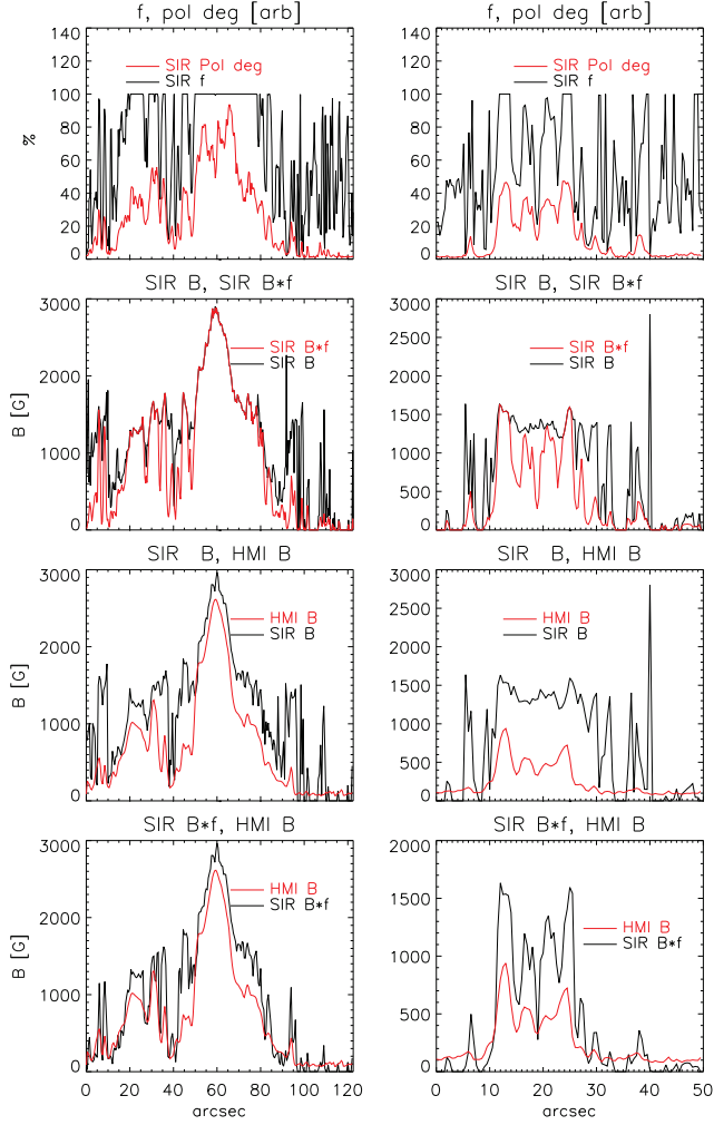
Figure 7. Different quantities along the spatial cuts across an umbra (left column) and a plage region (right column) marked in Fig. 6. Top to bottom: fill factor f (black lines) and polarization degree p (red lines), field strength B (black lines) and effective total flux Bf (red lines) in SP data, field strength in SP (black lines) and HMI data (red lines), and Bf in SP data (black lines) and B in HMI data (red lines).
