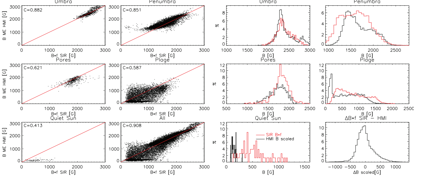
Figure 10. Scatterplots and histograms of Bf in SP and upscaled HMI B data. Same layout as in Fig. 4.
