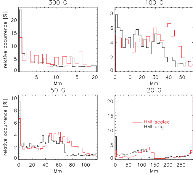
Figure 23. Histograms of the height of different magnetic field strength values. Clockwise, starting at lower right panel: for B = 20, 50, 300 and 100 G. Black (red) lines: original (scaled) HMI data.
