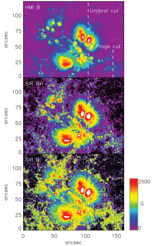
Figure 6. 2D maps of field strength SIR B (bottom panel) and total effective flux SIR Bf in SP data (middle panel), and field strength B in HMI data (top panel). The two vertical white dashed lines indicate the locations of spatial cuts across an umbra and a plage region shown in Figure 7.
