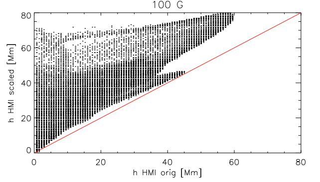
Figure 24. Scatter plot of the height with B = 100 G between original and scaled HMI data. The red line indicates unity slope.
