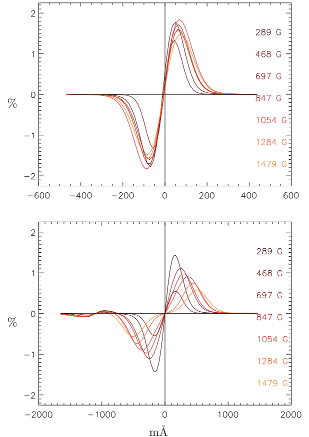
Figure 1. Synthetic FeI 1564.8 nm (bottom panel) and FeI 630.25 nm (top panel) Stokes V spectra for different field strengths (given at the right-hand side) and a varying magnetic fill factor.
