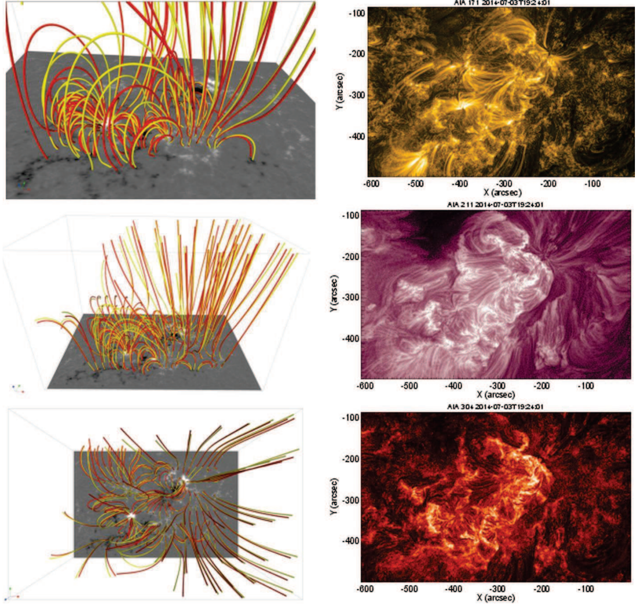
Figure 14. 3D views of the magnetic field extrapolation (left column) and concurrent AIA images (right column). Left column, bottom to top: top view of the extrapolation box with magnetic field lines from the same seed points before (red) and after scaling of the HMI magnetogram (yellow), side view (middle panel) and zoom on field lines of one spot and plage region (top panel). The background image shows HMI B_z . Right column, bottom to top: AIA images at 304, 211, and 171 Å.
