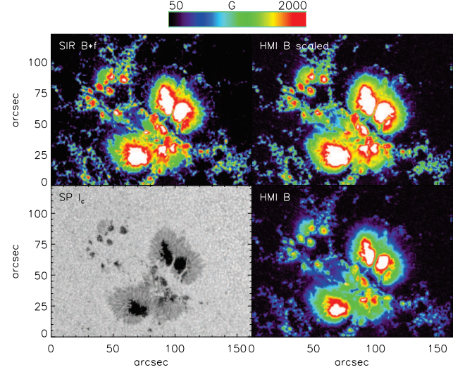
Figure 9. 2D maps of clockwise, starting left bottom: continuum intensity I_c and total effective flux Bf from SP, and upscaled and original field strength B from HMI.
