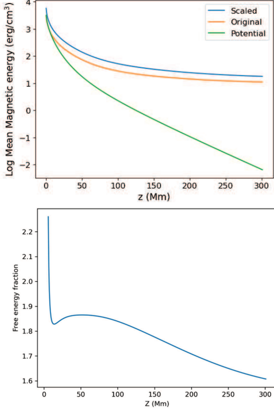
Figure 20. Mean magnetic energy (top panel) and ratio of the original and scaled free magnetic energy (bottom panel).
