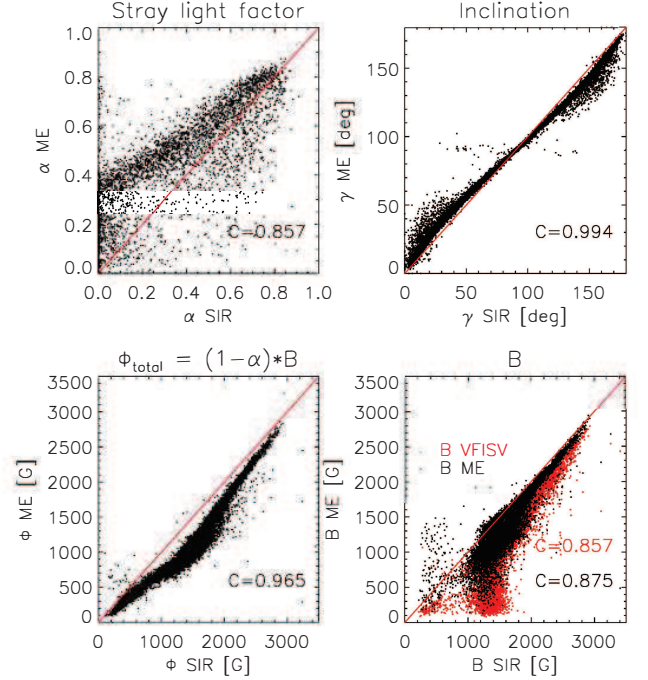
Figure 3. Scatterplots of quantities in the ME and SIR inversion of the SP data. Clockwise, starting left top: stray light factor \alpha , inclination \gamma , field strength B , and effective total flux Bf . The red lines indicate a unity slope. The linear correlation coefficients are given in the bottom right corner of each panel. The red dots in the lower right panel correspond to the VFISV ME inversion and were overplotted as second layer to enhance their visibility.
