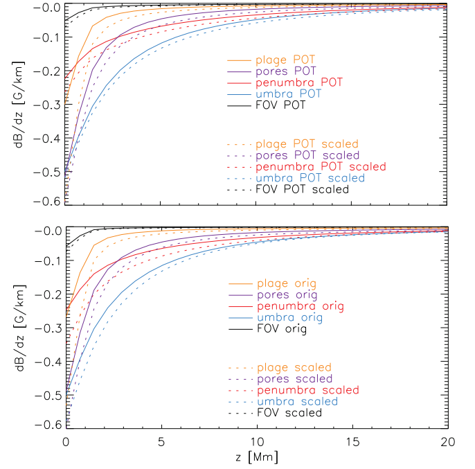
Figure 19. Gradient of magnetic field strength dB/dz for different structures. Bottom panel: NFFF extrapolation. Top panel: potential field extrapolation. Black: full FOV. Blue: umbra. Red: penumbra. Purple: pores. Orange: plage. The solid (dashed) lines show the original (scaled) HMI data.
